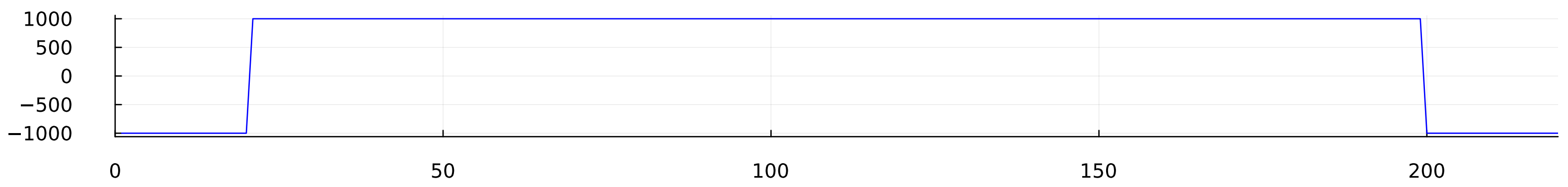
h(Z_{hyp}=880)
