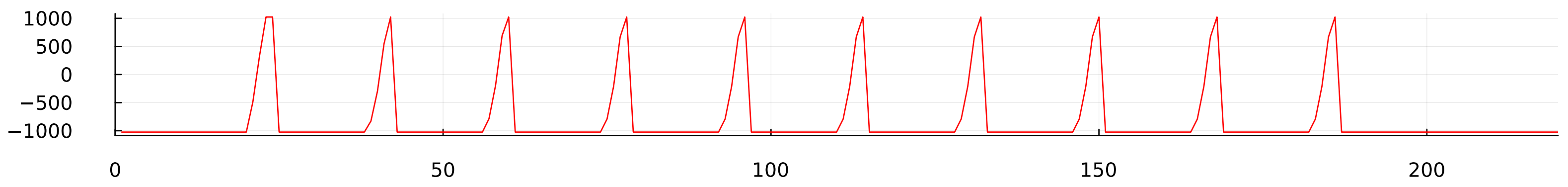
h(Z_{hyp}=900)
